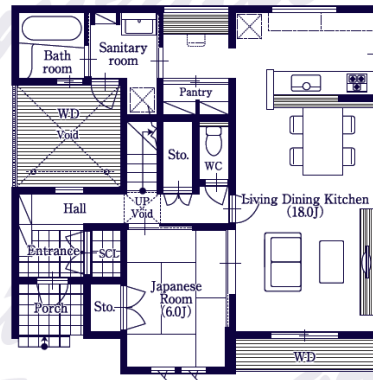
▶ The first floor plan view
